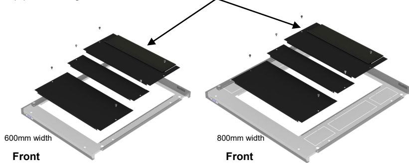
Top panel configuration (800D shown)
